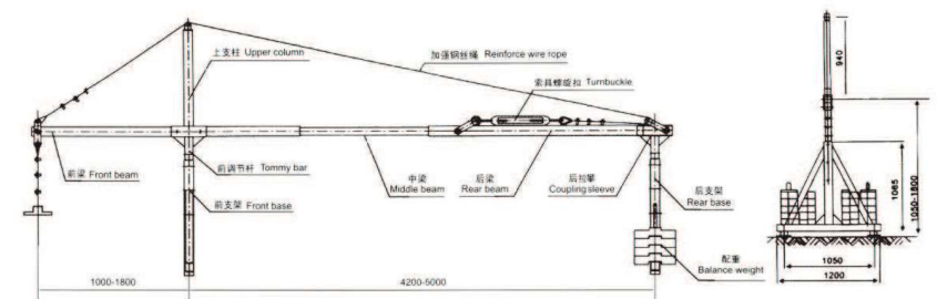
ZLP系列悬挂机构名称及规格 ZLP series high operation suspending part name and size
