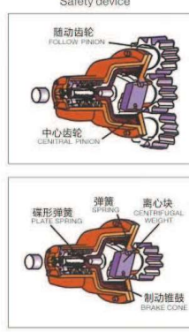
防坠安全锁 Safety device
