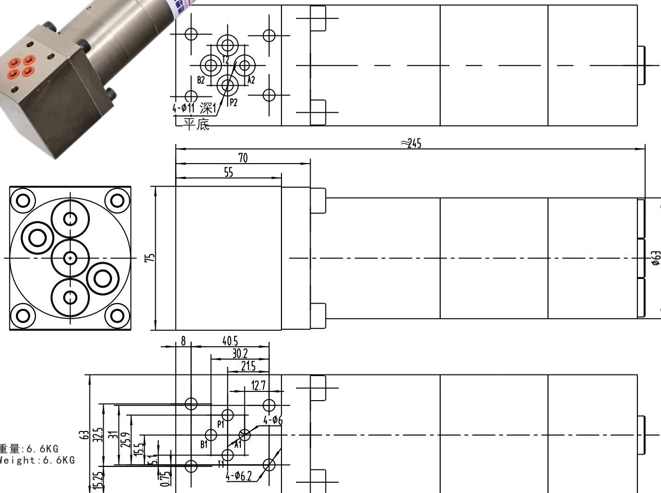
叠加式安装尺寸(DA/P/G) Dimensions of Stacking Manifold
