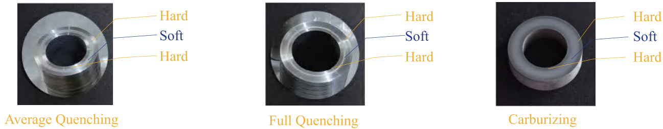
Cut Surface Photo of Track Pin
