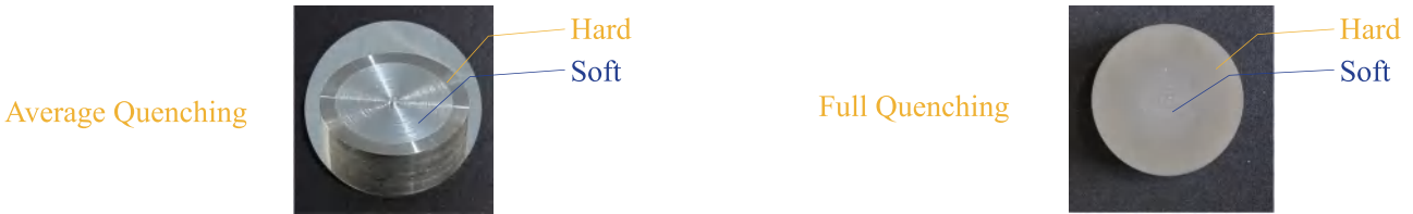
Cut Surface Photo of Track Pin
