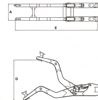
ONE-WAY TYPE — WCA20S
