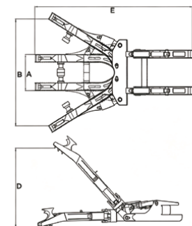
TWO-WAY TYPE — WCA20D
