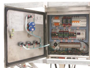
3-phase
