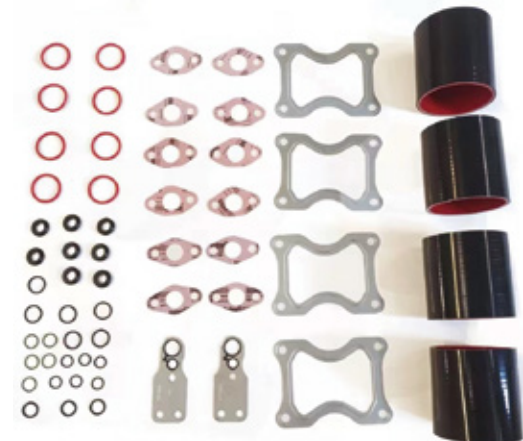
QSK60涡轮增压器中冷器修理包4089233 Turbocharger Intercooler Gasket Kit
