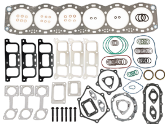
S60发动机上修理包(全配)23536443 Upper Gasket Kit
