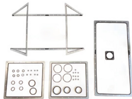
QSK60油底壳垫片修理包4956000 Oil Pan Gasket Kit
