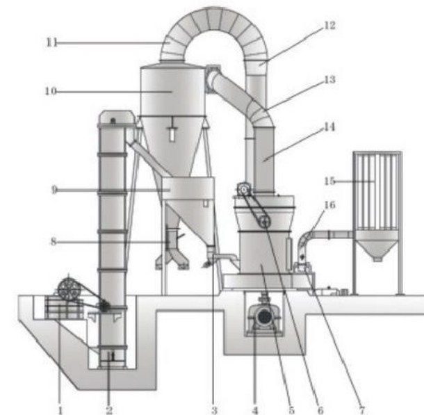
Schematic diagram of supporting equipment
