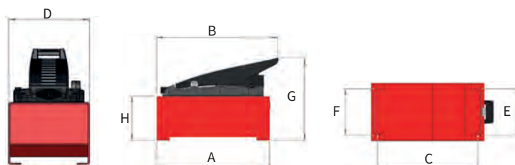
AHP1121, AHP1141 (钢制油箱)
