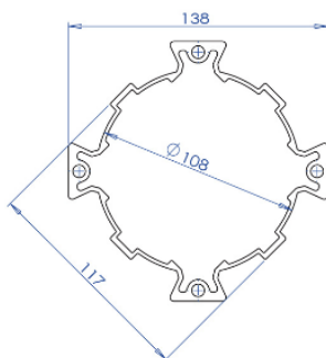
DETAIL OUTER TUBE
