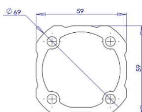
DETAIL INNER TUBE
