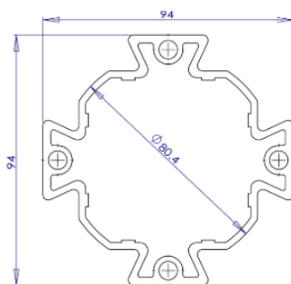
DETAIL OUTER TUBE
