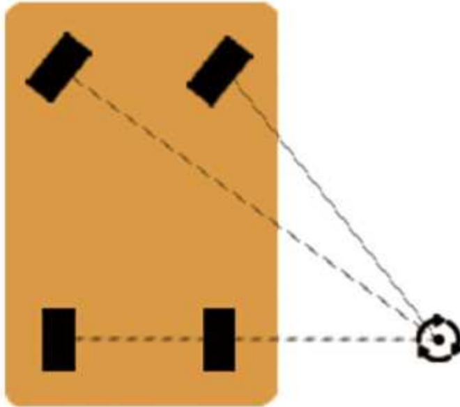
右转 Turn right
