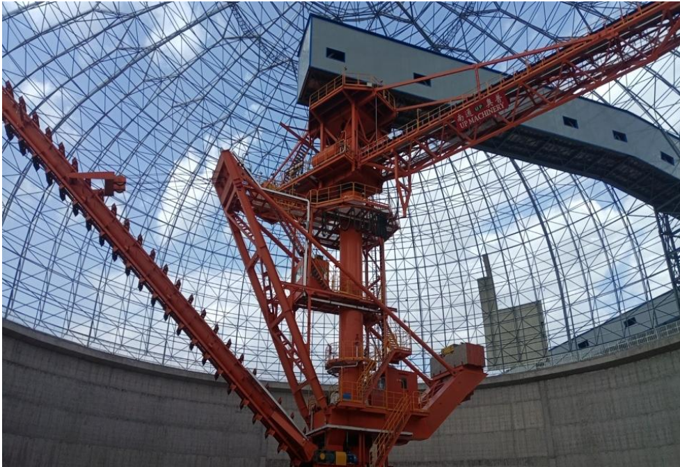
圆形顶堆侧取 (门架式、配重式、桥式) Circular top-stacking side-reclaiming (portal, counterweight, bridge type)
