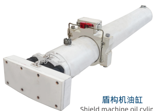
推进油缸 Propulsion cylinder
