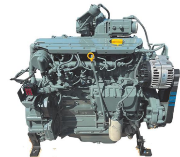
TCD2013 L4 4-Cylinders Displacement:4.8L Power:70-104KW Water-cooled 4-stroke
