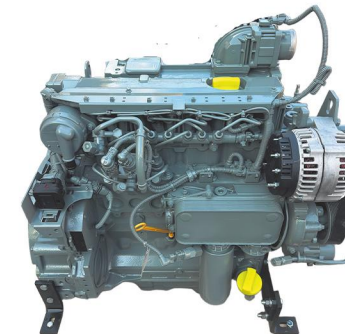
TCD2012 L4 4-Cylinders Displacement:4L Power:66-103KW Water-cooled 4-stroke
