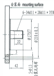
XWM3- \star\star SL 1
