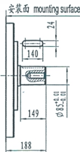
标准平键XWM71-**-**B stand flat key shaft
