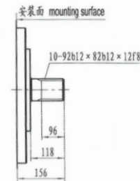
标准外花键XWM31-** stand external splined shaft
