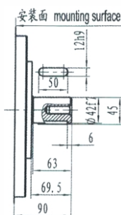
标准平键XWM6-**B stand flat key shaft
