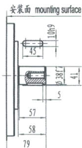
标准平键XWM3-**B stand flat key shaft
