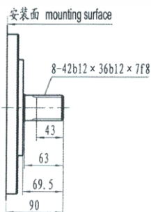
标准外花键XWM6-** stand external splined shaft
