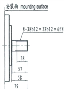
标准外花键XWM3-** stand external splined shaft
