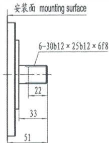
标准外花键 XWM1-** stand external splined shaft
