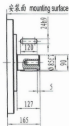
标准平键XWM31-**B stand flat key shaft
