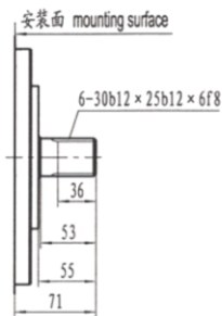
标准外花键XWM2-** stand external splined shaft
