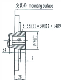
标准内花键XWM6-**I stand internal splined shaft
