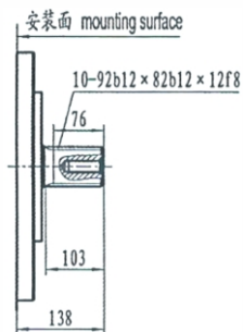
标准外花键XWM71-**-** stand external splined shaft
