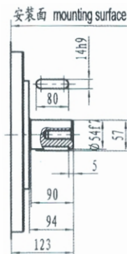
标准平键XWM8-**B stand flat key shaft
