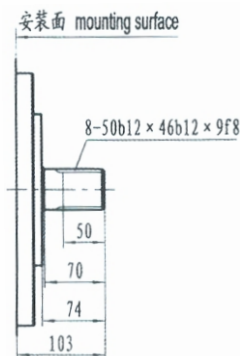
标准外花键XWM8-** stand external splined shaft
