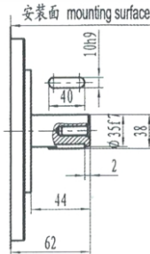
标准平键 XWM1-**B stand flat key shaft
