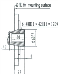
标准内花键XWM3-**1 stand internal splined shaft
