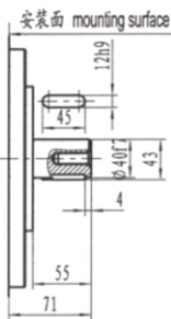
标准平键XWM2-**B stand flat key shaft
