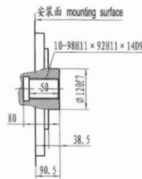
标准内花键XWM31-**I stand internal splined shaft
