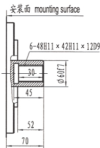
标准内花键XWM2-**1 stand internal splined shaft
