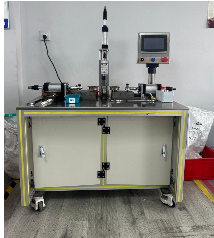
Riveting machine
