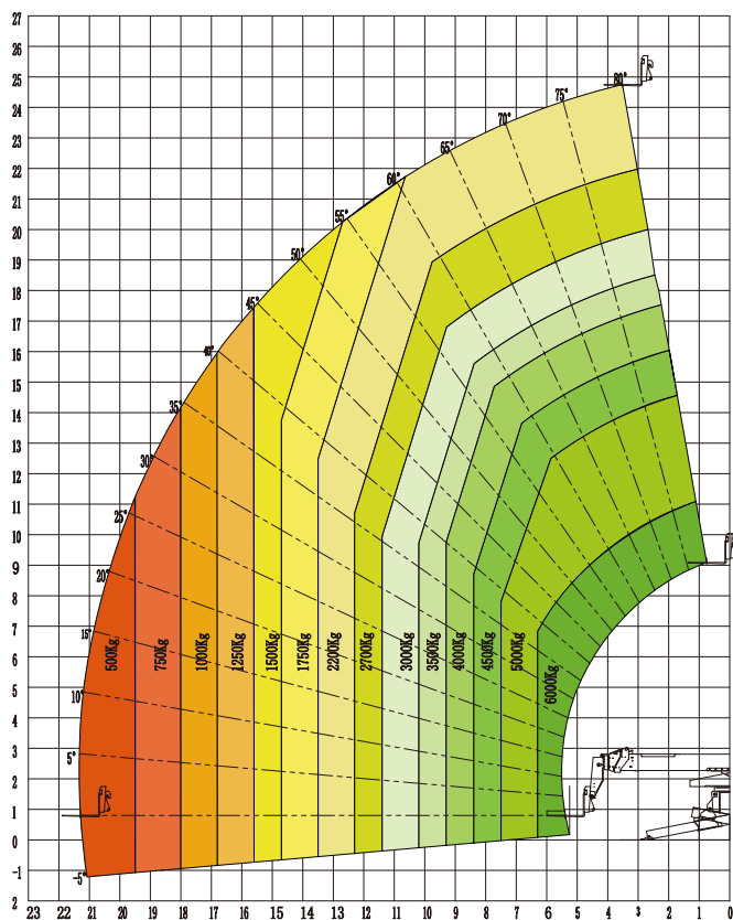
RT6025载荷表(支腿放下)
