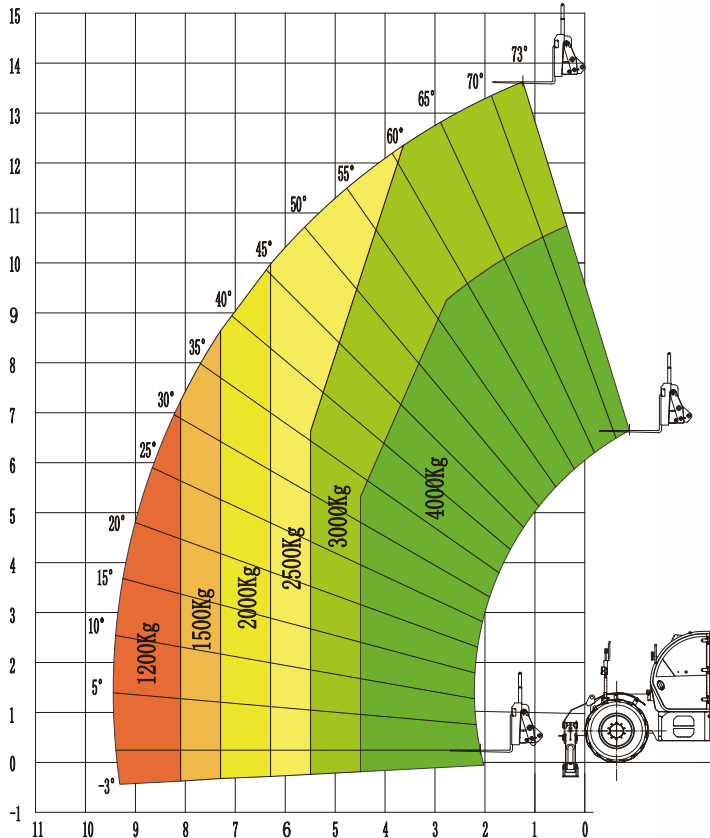
T4014载荷表(支腿放下)
