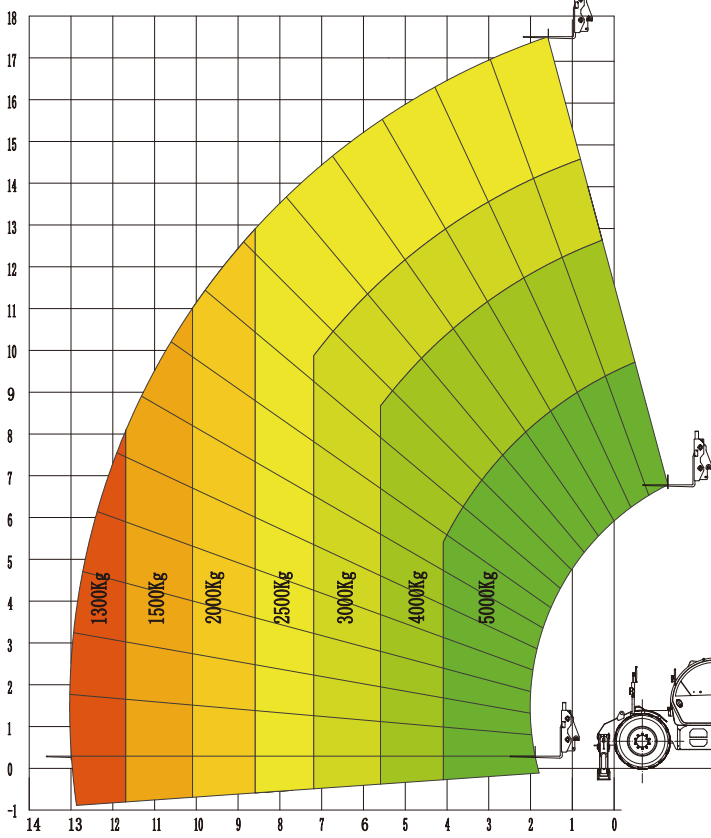
T5018载荷表(支腿放下)
