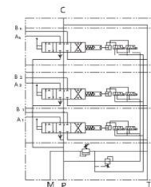
电液控 Electro-hydraulic control
