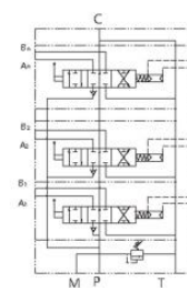
气控 Pneumatic control
