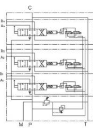
电液控 Electro-hydraulic control
