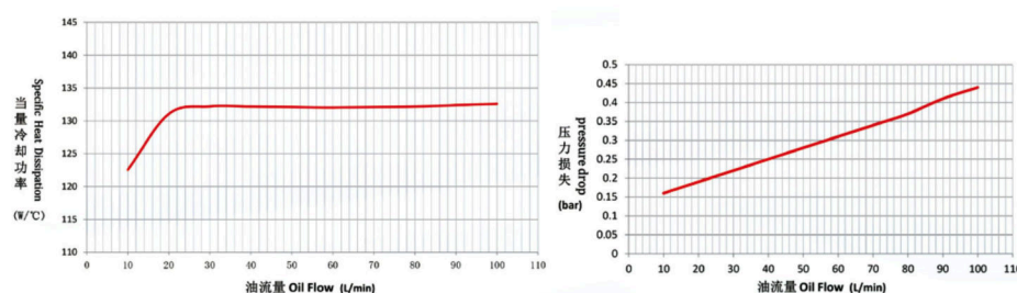
性能曲线 PERFORMANCE CURVE
