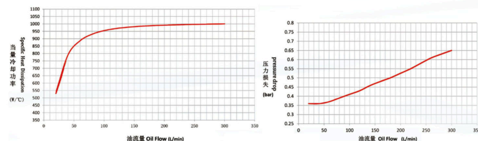
性能曲线 PERFORMANCE CURVE
