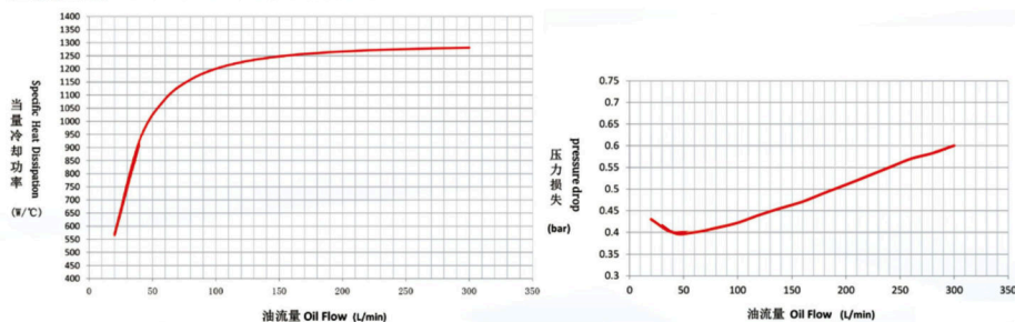
性能曲线 PERFORMANCE CURVE
