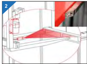
Fork camera The camera system is equipped on the fork, which provides a better view during fork moving, avoid the problems that view may be blocked by the pallet feet while stacking. The camera is made of stainless steel, IP protection grade is IP69, the shockproof grade is 10G. Not afraid of bump.
