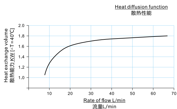
性能曲线 PERFORMANCE CURVE
