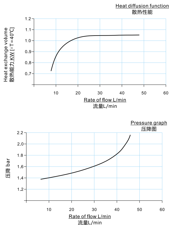
性能曲线 PERFORMANCE CURVE
