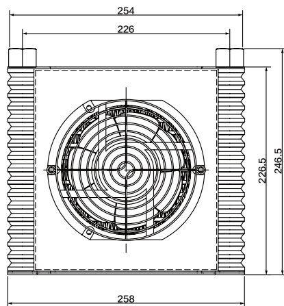
产品线图 PRODUCT LINE DIAGRAM
