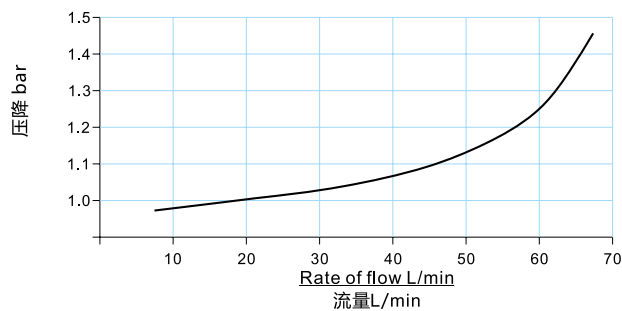
Pressure graph 压降图
