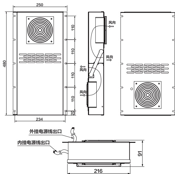
产品线图 PRODUCT LINE DIAGRAM
