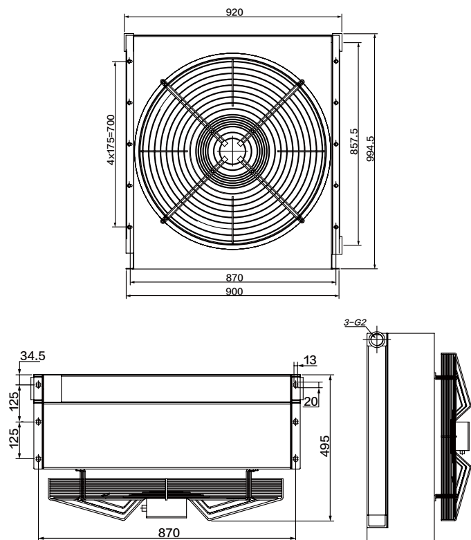
产品线图 PRODUCT LINE DIAGRAM
