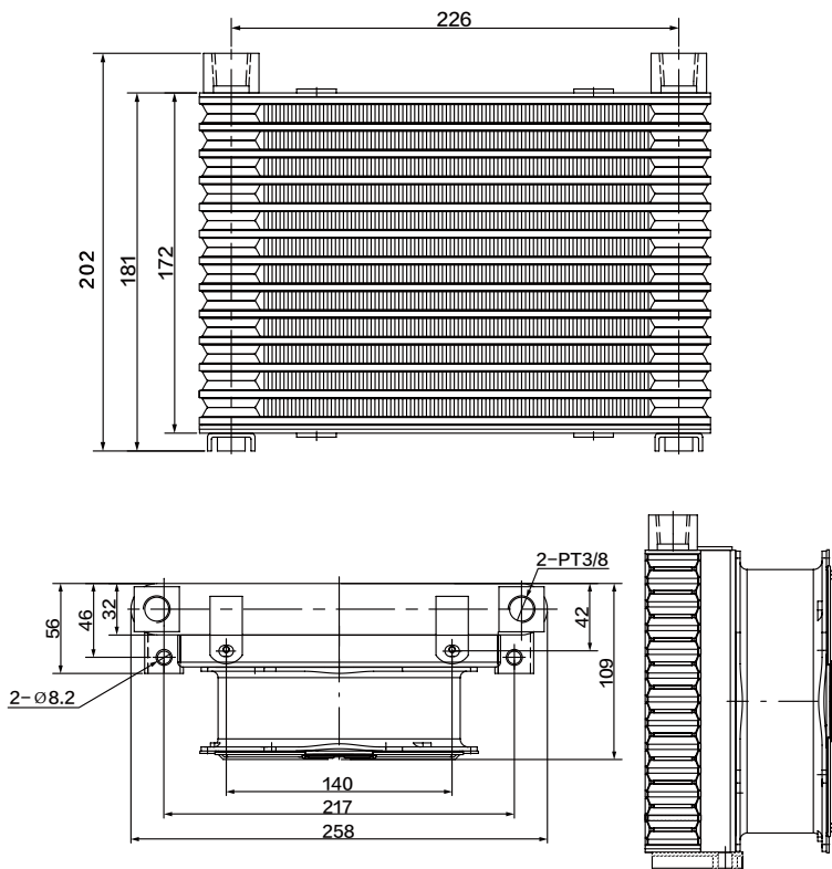
产品线图 PRODUCT LINE DIAGRAM
