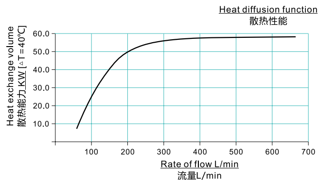
性能曲线 PERFORMANCE CURVE
