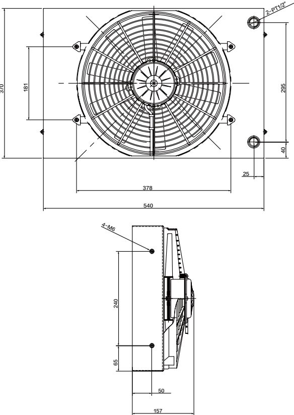
产品线图 PRODUCT LINE DIAGRAM
