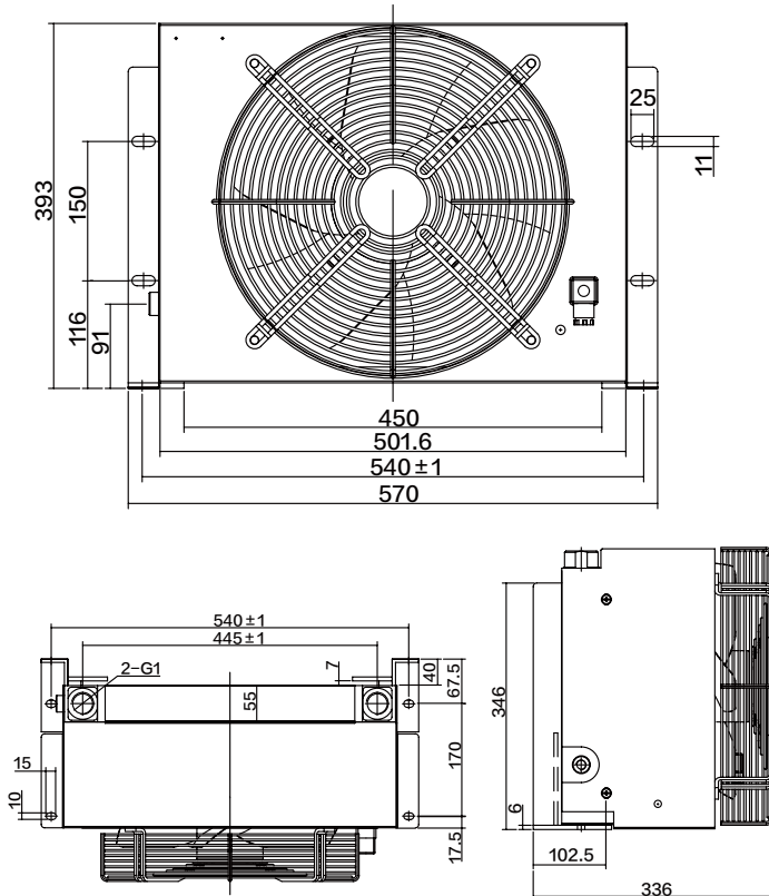
产品线图 PRODUCT LINE DIAGRAM
