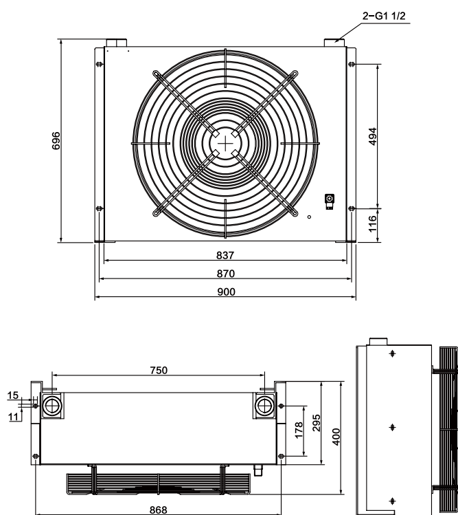
产品线图 PRODUCT LINE DIAGRAM
