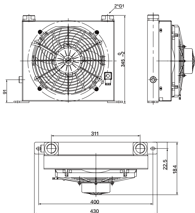
产品线图 PRODUCT LINE DIAGRAM
