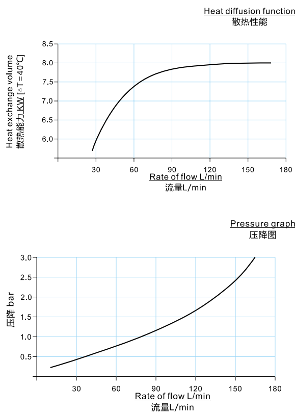
性能曲线 PERFORMANCE CURVE
