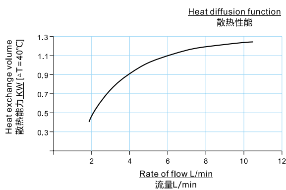
性能曲线 PERFORMANCE CURVE
