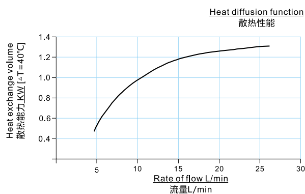
性能曲线 PERFORMANCE CURVE
