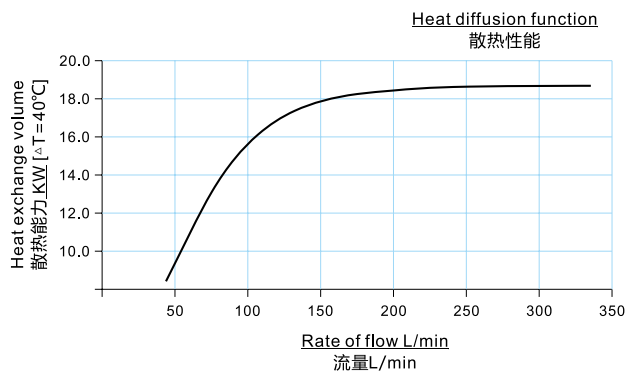
性能曲线 PERFORMANCE CURVE
