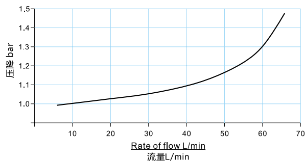
Pressure graph 压降图
