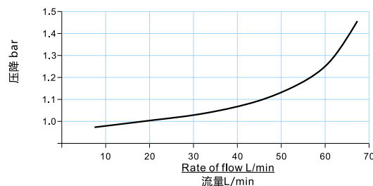
Pressure graph 压降图
