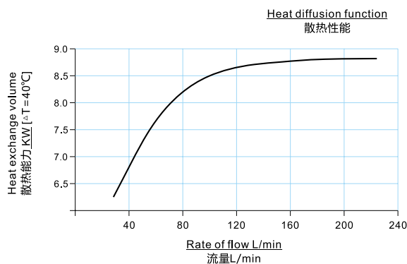
性能曲线 PERFORMANCE CURVE
