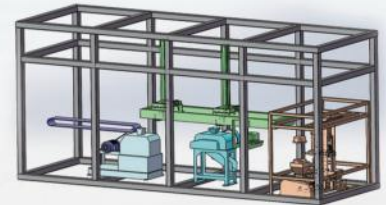
Automatic ore preparation machine
