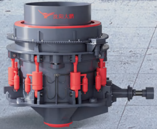
PYH multi cylinder hydraulic cone crusher
