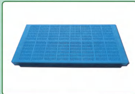
Non-continuous Slot Polyurethane Screen Panel
