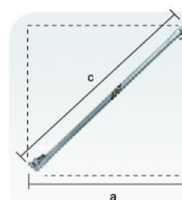
RFH-B001C(mm) 斜拉杆 Diagonal aXb c 732X2000 2119 1400X2000 2393 1572X2000 2451 2072X2000 2806 2572X2000 3137 3072X2000 3572 2572X1500 3434 2072X1500 2845 2572X1000 2616 2072X1000 2162 Φ48.3x2.5mm
