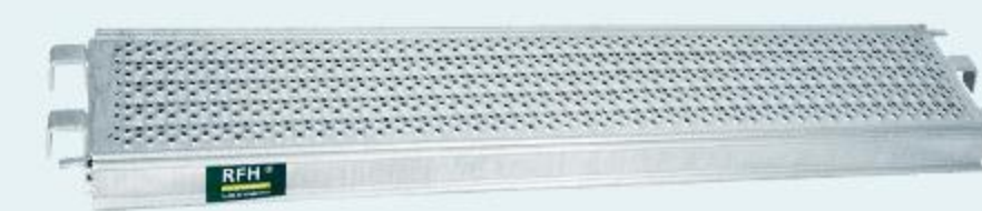
RFH-B006I 脚踏板 Scaffold Plank 739,1065,1500,2000,2500,3000 (mm) (320x76x1.5mm 300x76x1.2mm)
