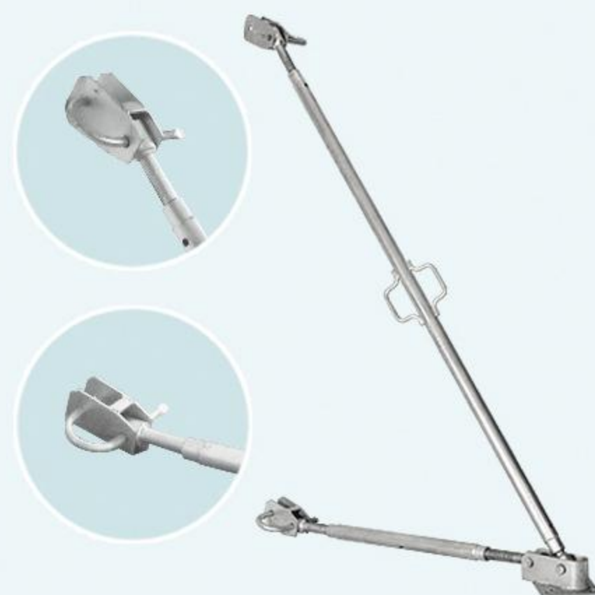
RFH-FW00GA 重型推拉支撑 Push-Pull Shore 17.5Kg 610-900mm 1600-1700mm
