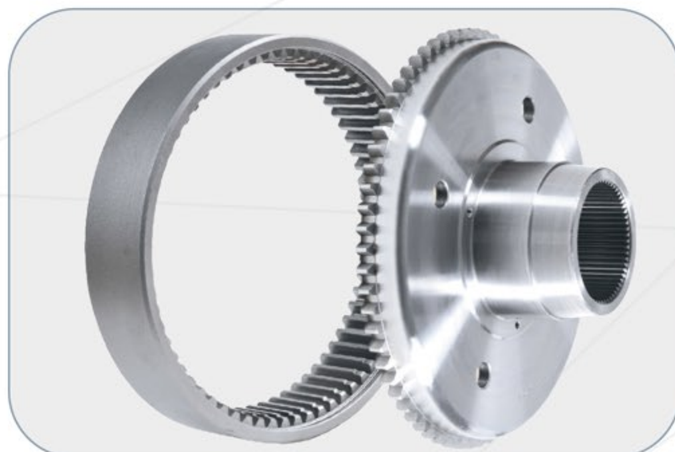
XCMG 67 INTERNAL INTERNAL GEAR RING SUPPORTING PLATE (徐工 67齿内齿圈 支承盘)
