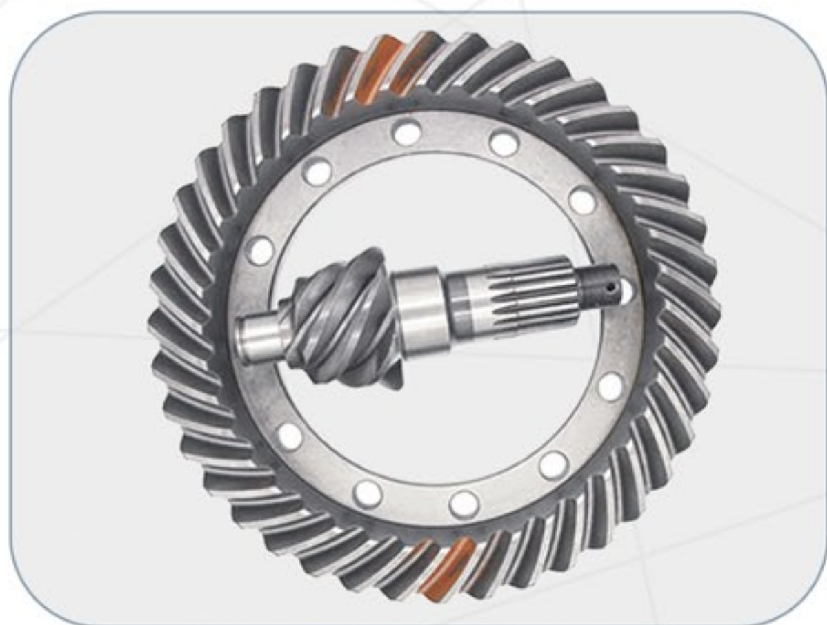
MITSUBISHI PS125
