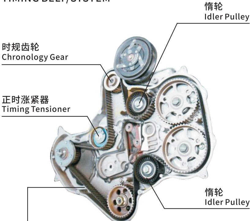
正时皮带 Timing Belt
