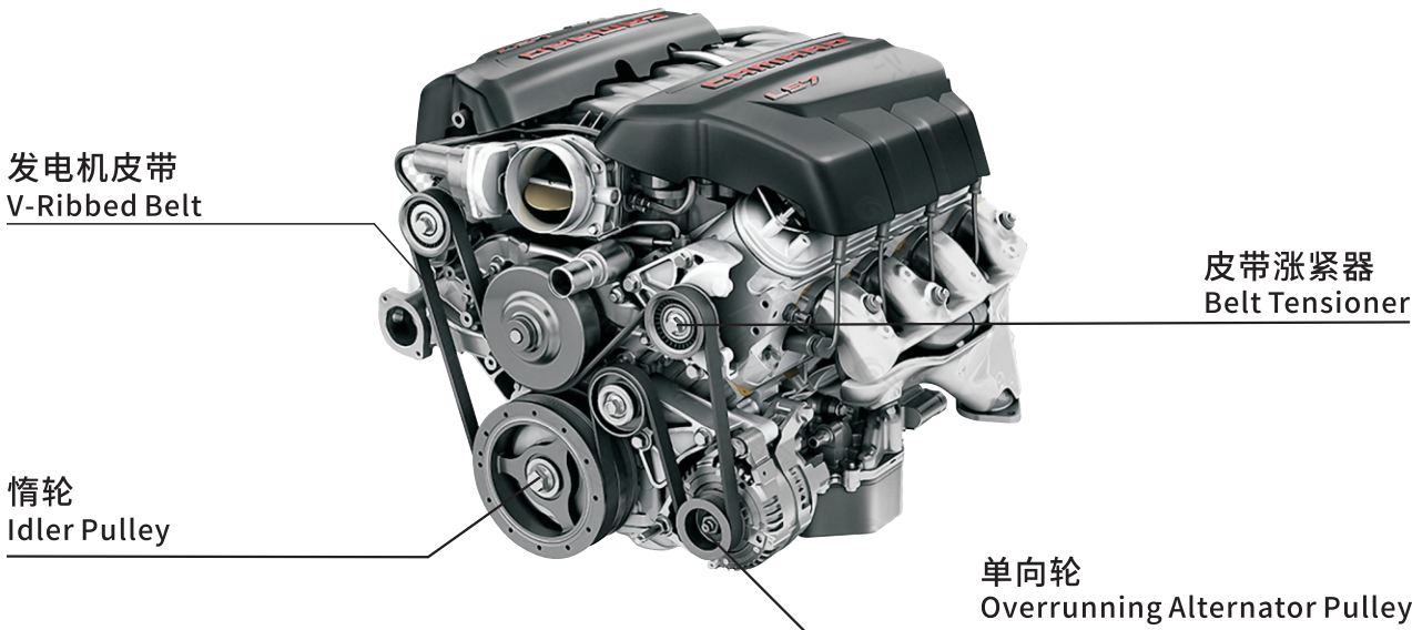
单向轮 Overrunning Alternator Pulley
