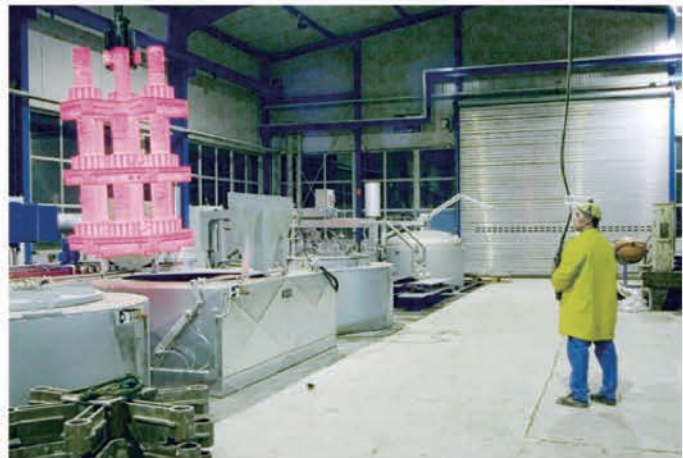
批量油冷 Oil Cooling in Large Volume
