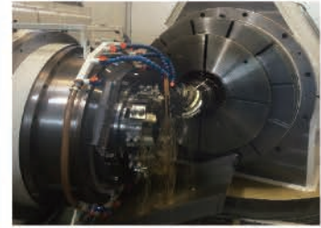
Hard Cutting 硬切齿
