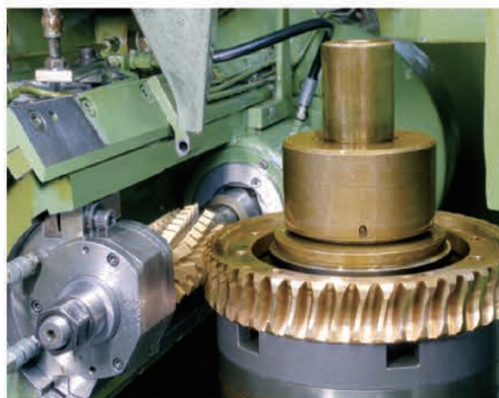
蜗轮铣削 Milling of Worm Gear
