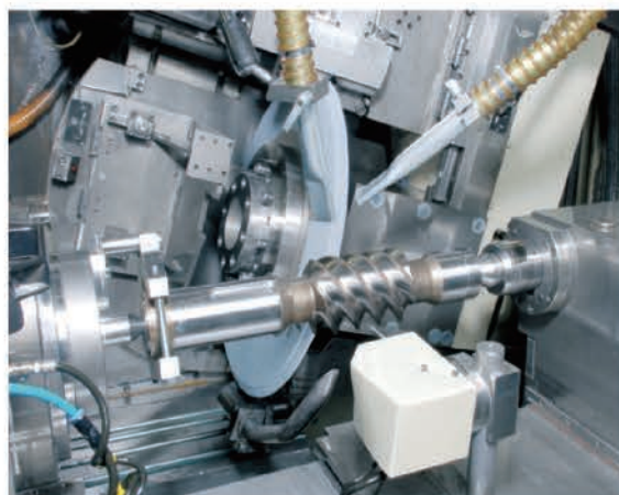
蜗轮研磨 Grinding of Worm Gear
