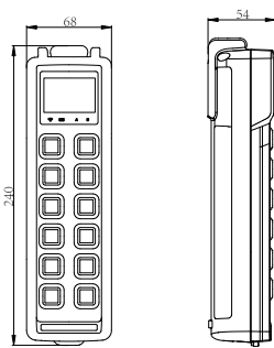
T-F3 Series size
