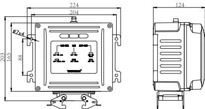
MMN Series Size
