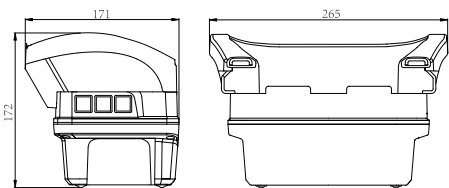
T-F4 Series size
