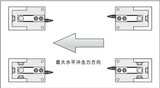
矩形布置
