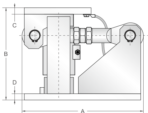
PROFILE
