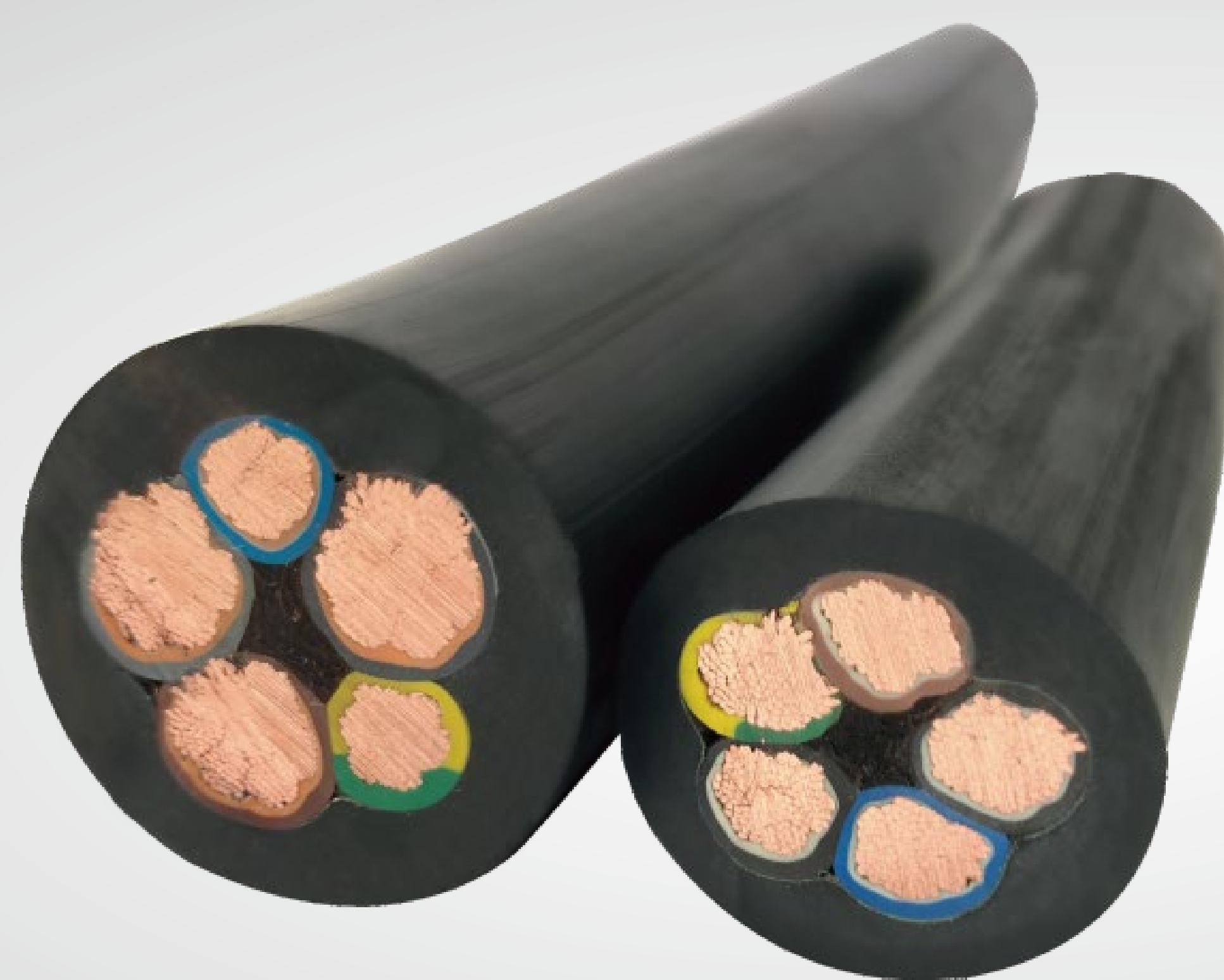
通用橡套软电缆 Rubber Sheath Flexible Cable For Communication
