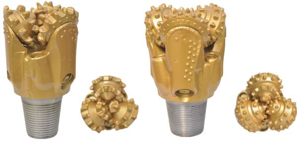
Roller Cone Pilot Bit
