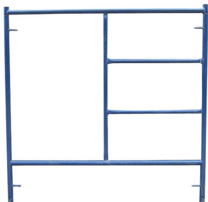
梯型门架 Ladder Frame Ø42X2.3mm
