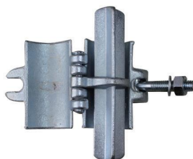
锻压内接扣件 Forged Inner Joint 48.3mm 1.35kg
