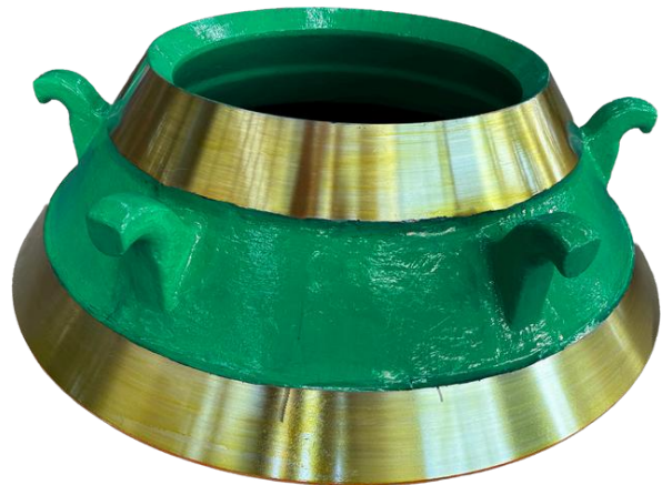
轧臼壁Bowl Liner
