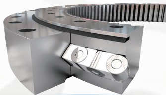
3.Single row crossed roller slewing bearing
