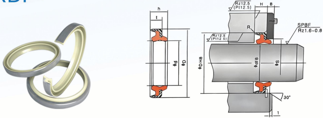
DKB Dust seal
