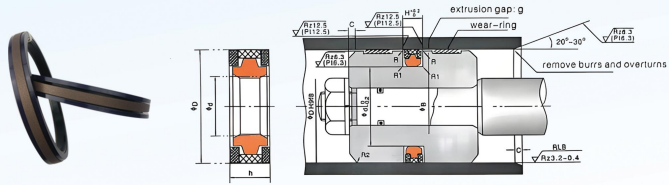
SPGW Piston seal
