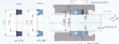
IDI T YOE ROD SEAL(RECIPROCATING)
