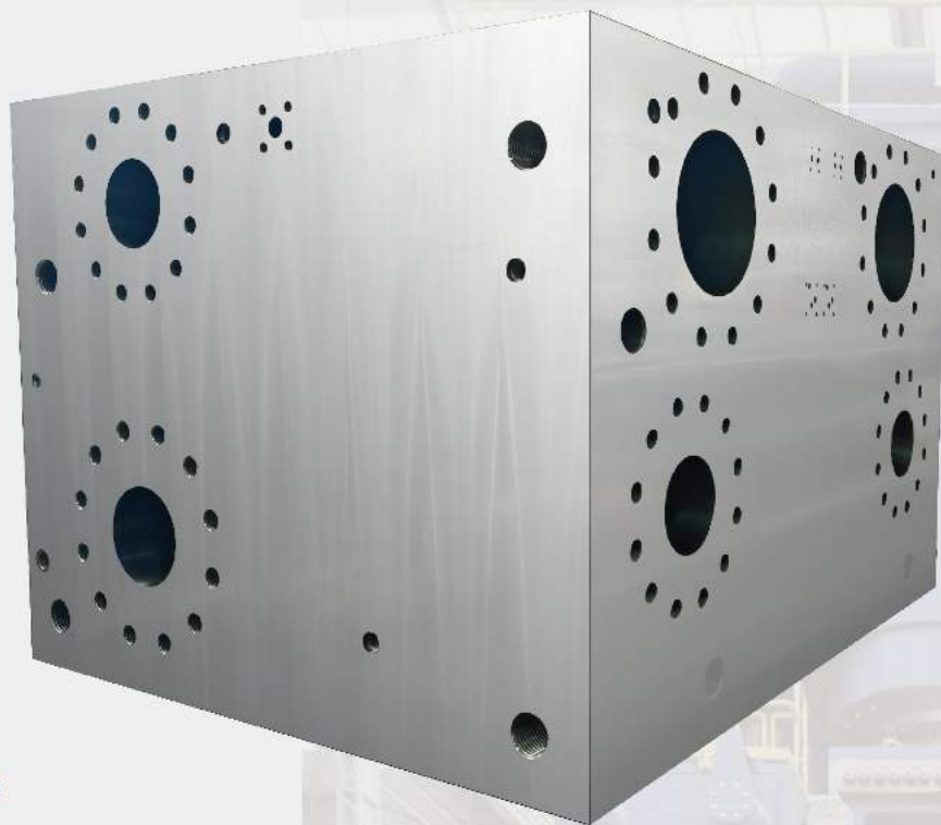
► 185 MN 快锻机主阀块 Manifold for 185MN high-speed forging press
