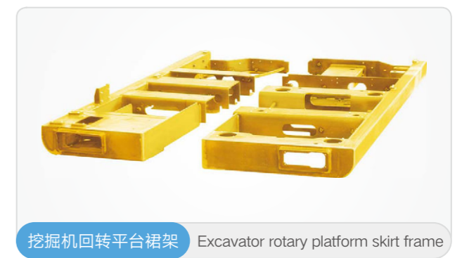
挖掘机下车架履带梁 Excavator undercarriage crawler belt beam
