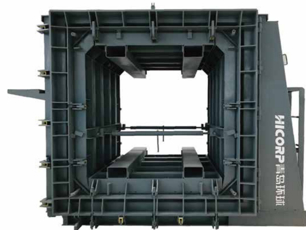
综合管廊模具 Precast Concrete Box Culvert Mold
