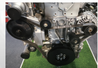
同步带 Timing V-belt
