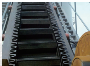
大倾角输送带 Sidewall Conveyor Belt
