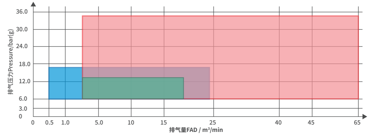
志高螺杆主机功能覆盖图 Screw air end capacity coverage
