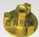
XIN-B005C 火索帽螺母 Wing Nut 0.58kg/Dia90mm
