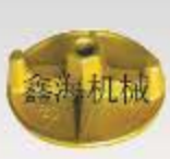
XIN-B006 锻压火索帽螺母 Forged Wing Nut 1.25kg/Dia130mm
