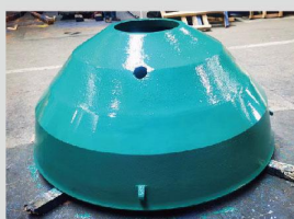
Mantle 动锥
