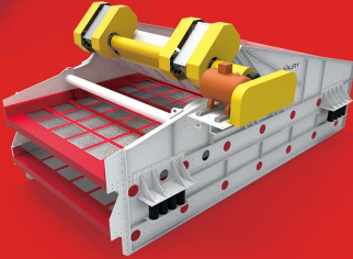
圆振筛-双层
