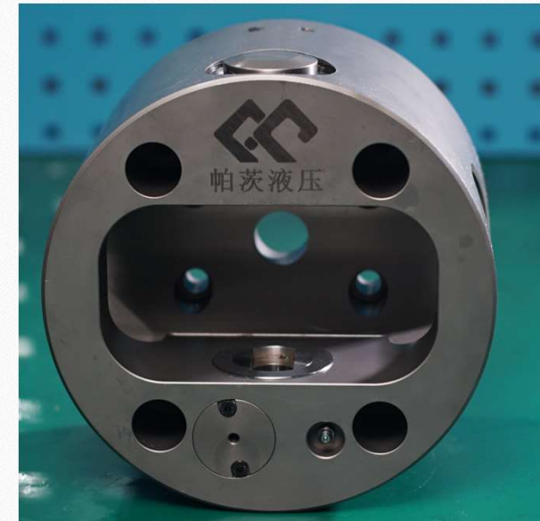
Self-Developed index chuck 自主研发的分度卡盘
