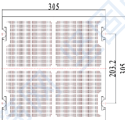
筛板安装结构图 Structural drawing of Screen Board Installation
