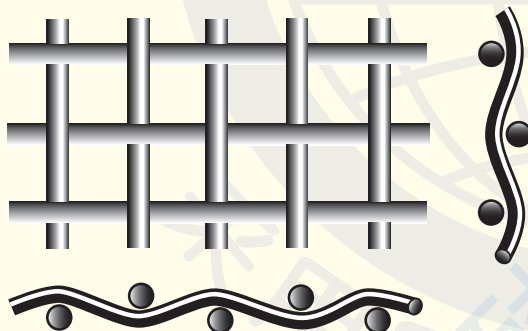
C 型 - 双向隔波弯曲筛网 Type C: Double-way Separated Curved Mesh
