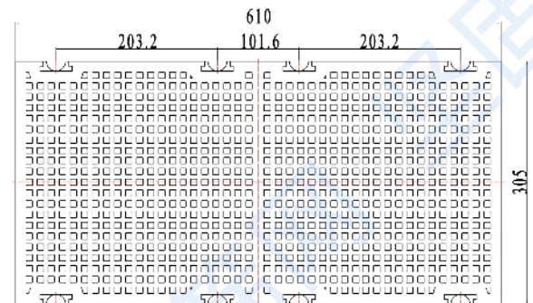
筛板安装结构图 Structural drawing of Screen Board Installation
